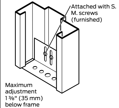
Adjustable Base Anchor
