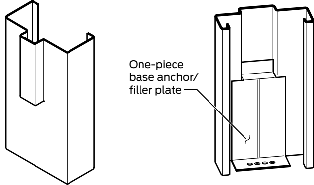
90° hospital stops
