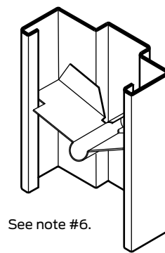
Existing Masonry Anchor
