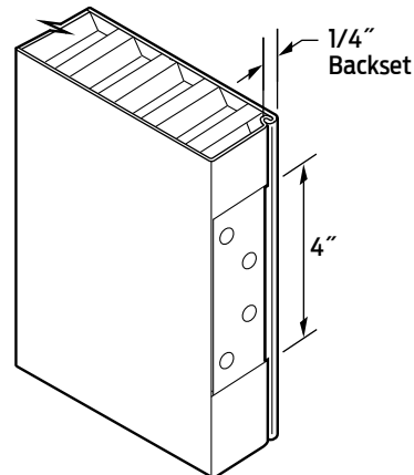
4" Hinge Detail L20 & CE 20 Series Only
